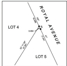
DETAIL A SCALE OF ENLARGEMENT IS 1:100 AT THE INTENDED PLOT SIZE OF PLAN
